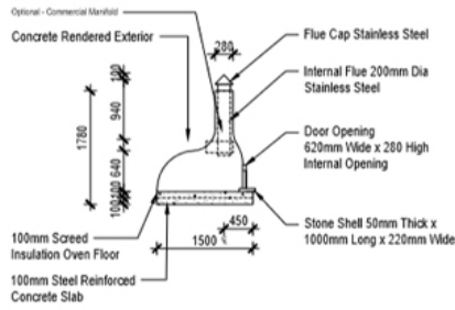
Donatello Side Elevation
