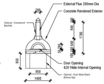
Donatello Front Elevation
