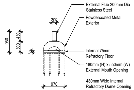
Giotto Front Elevation
