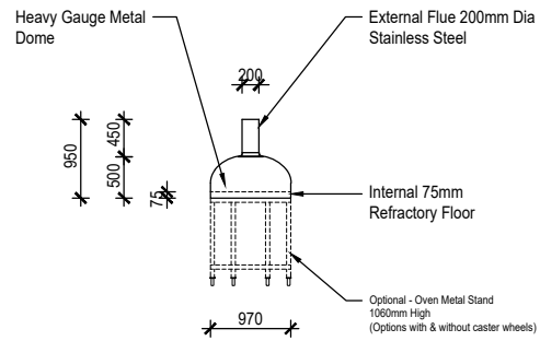
Giotto Rear/Side Elevation
